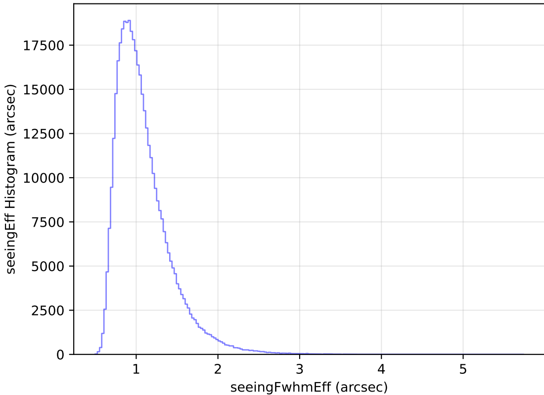
too_elab_r32_d2_ugrizy_v3.4_10yrs All sky z band: seeingEff Histogram
