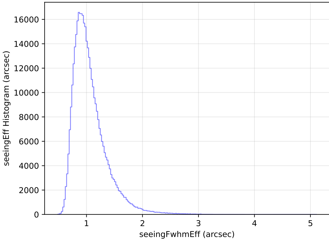
too_elab_r32_d2_ugrizy_v3.4_10yrs All sky y band: seeingEff Histogram
