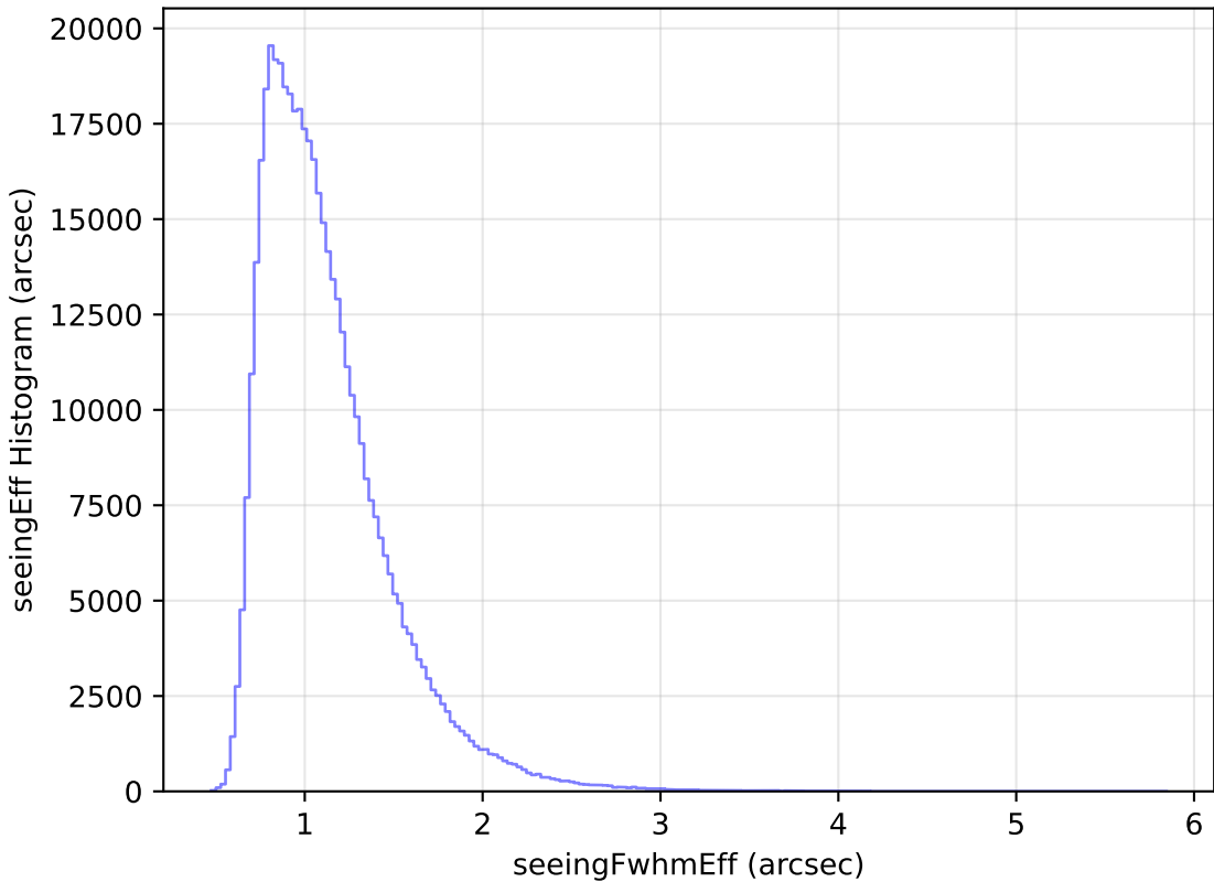
too_elab_r32_d2_ugrizy_v3.4_10yrs All sky r band: seeingEff Histogram
