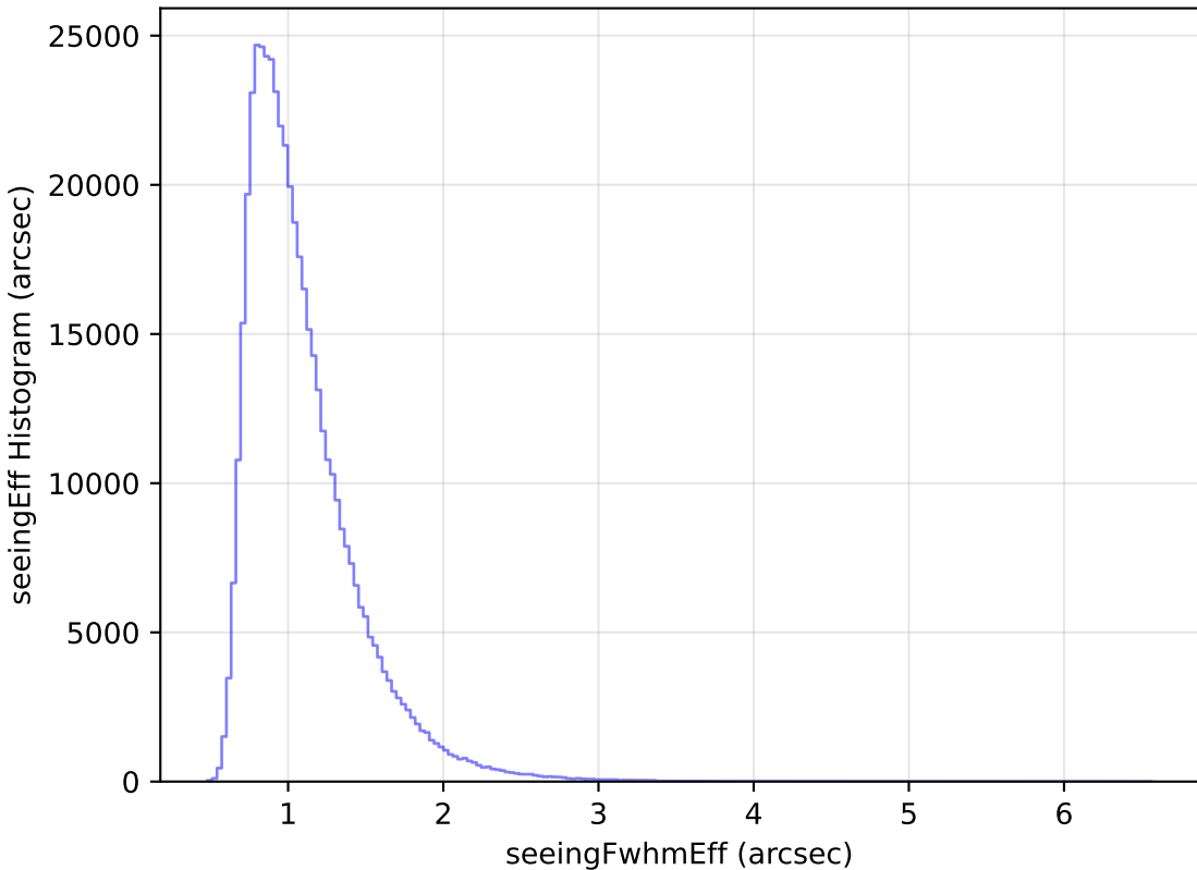
too_elab_r32_d2_ugrizy_v3.4_10yrs All sky i band: seeingEff Histogram
