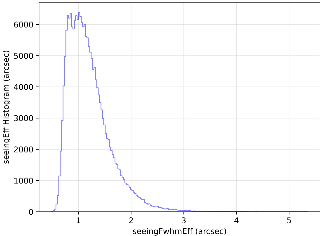
too_elab_r32_d2_ugrizy_v3.4_10yrs All sky g band: seeingEff Histogram
