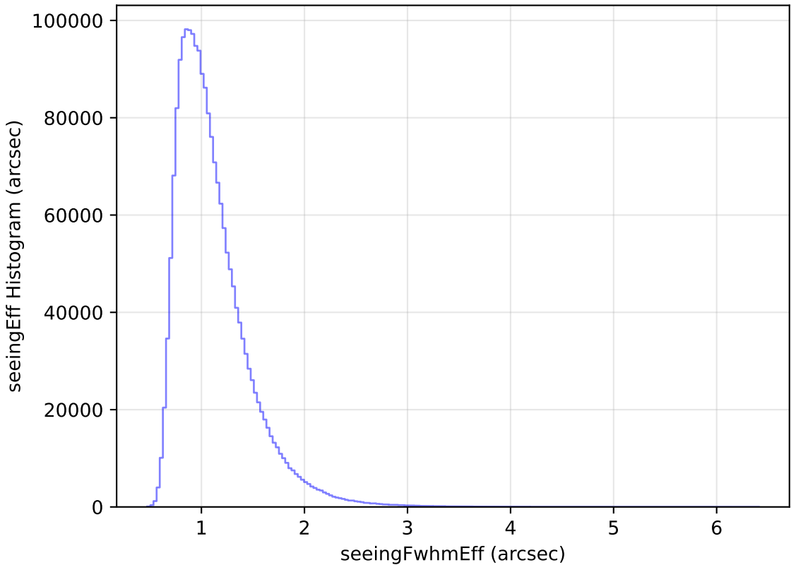
too_elab_r32_d2_ugrizy_v3.4_10yrs All sky all bands: seeingEff Histogram
