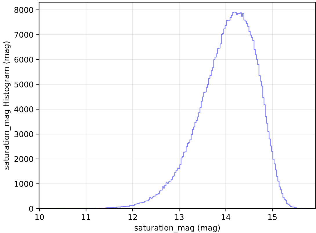
too_elab_r32_d2_ugrizy_v3.4_10yrs WFD z band: saturation_mag Histogram
