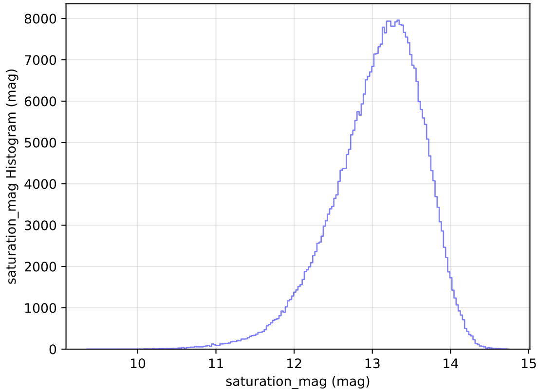
too_elab_r32_d2_ugrizy_v3.4_10yrs WFD y band: saturation_mag Histogram
