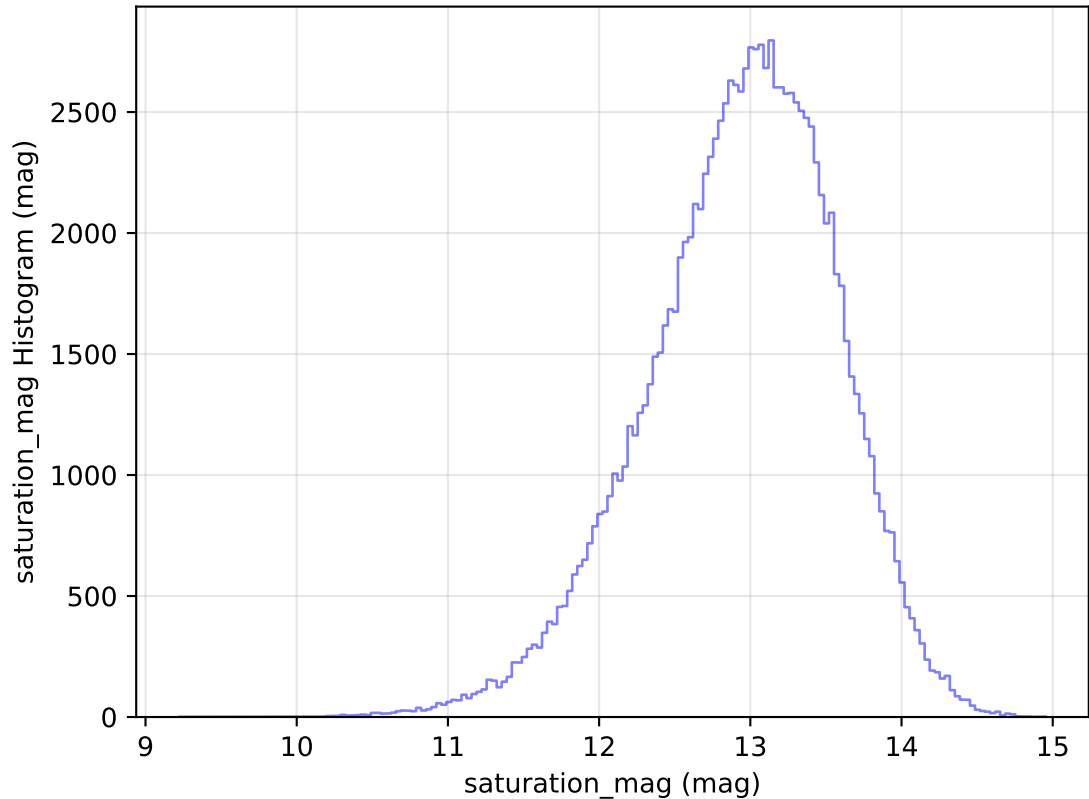
too_elab_r32_d2_ugrizy_v3.4_10yrs WFD u band: saturation_mag Histogram
