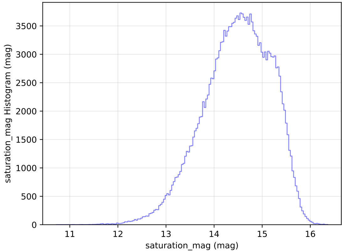
too_elab_r32_d2_ugrizy_v3.4_10yrs WFD g band: saturation_mag Histogram
