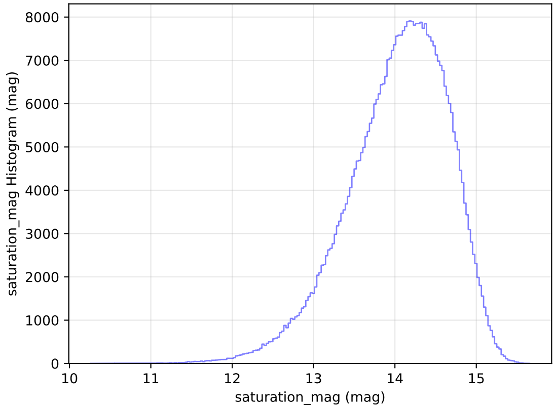
too_elab_r32_d2_ugrizy_v3.4_10yrs All sky z band: saturation_mag Histogram
