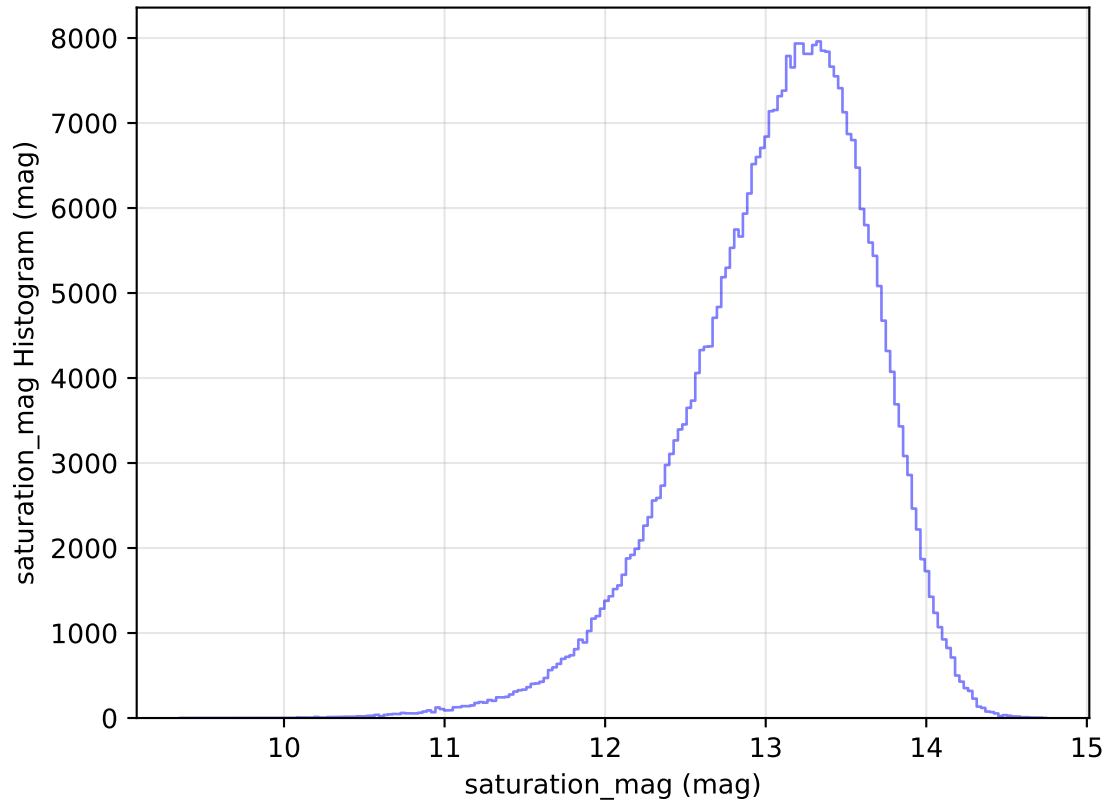
too_elab_r32_d2_ugrizy_v3.4_10yrs All sky y band: saturation_mag Histogram
