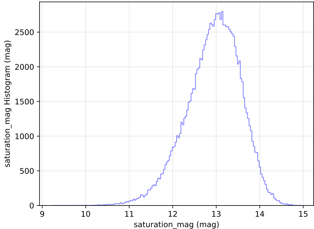
too_elab_r32_d2_ugrizy_v3.4_10yrs All sky u band: saturation_mag Histogram
