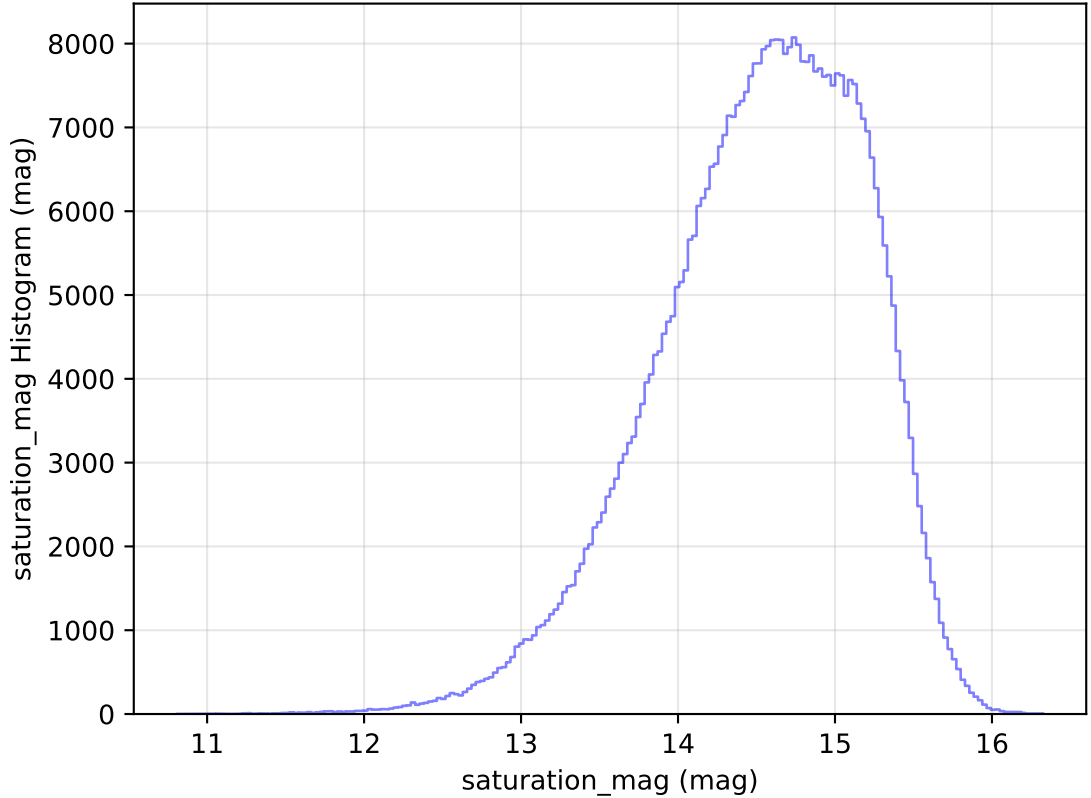
too_elab_r32_d2_ugrizy_v3.4_10yrs All sky r band: saturation_mag Histogram
