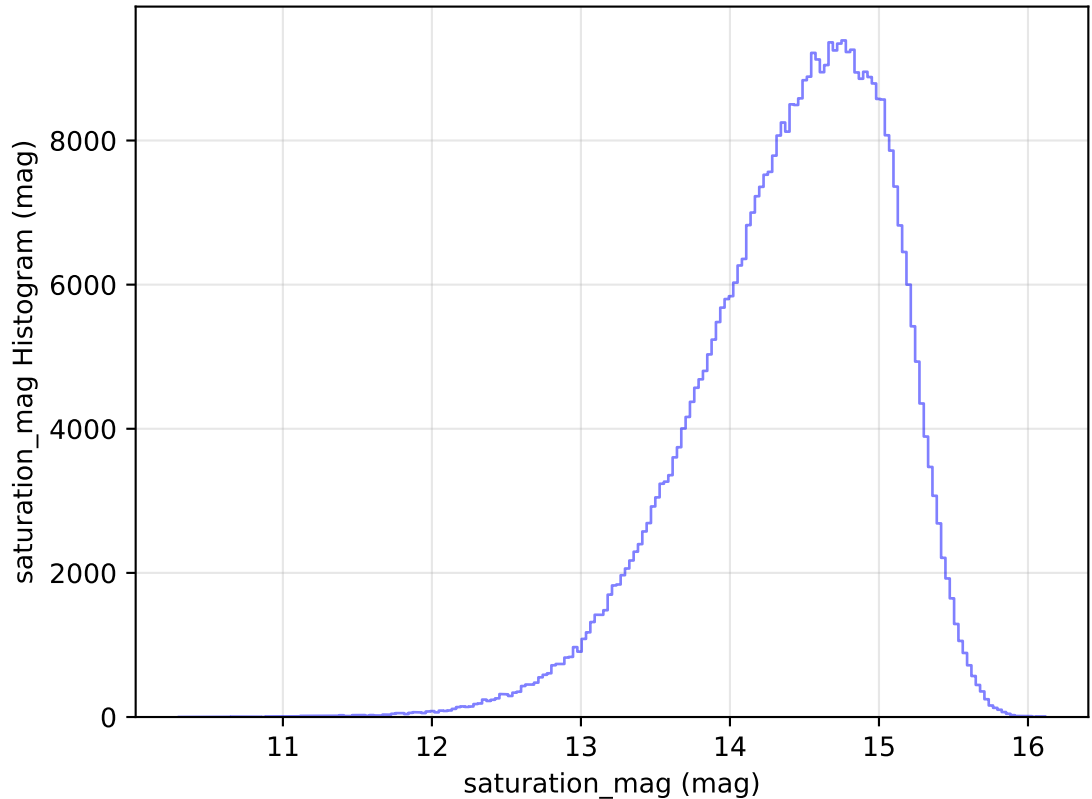
too_elab_r32_d2_ugrizy_v3.4_10yrs All sky i band: saturation_mag Histogram
