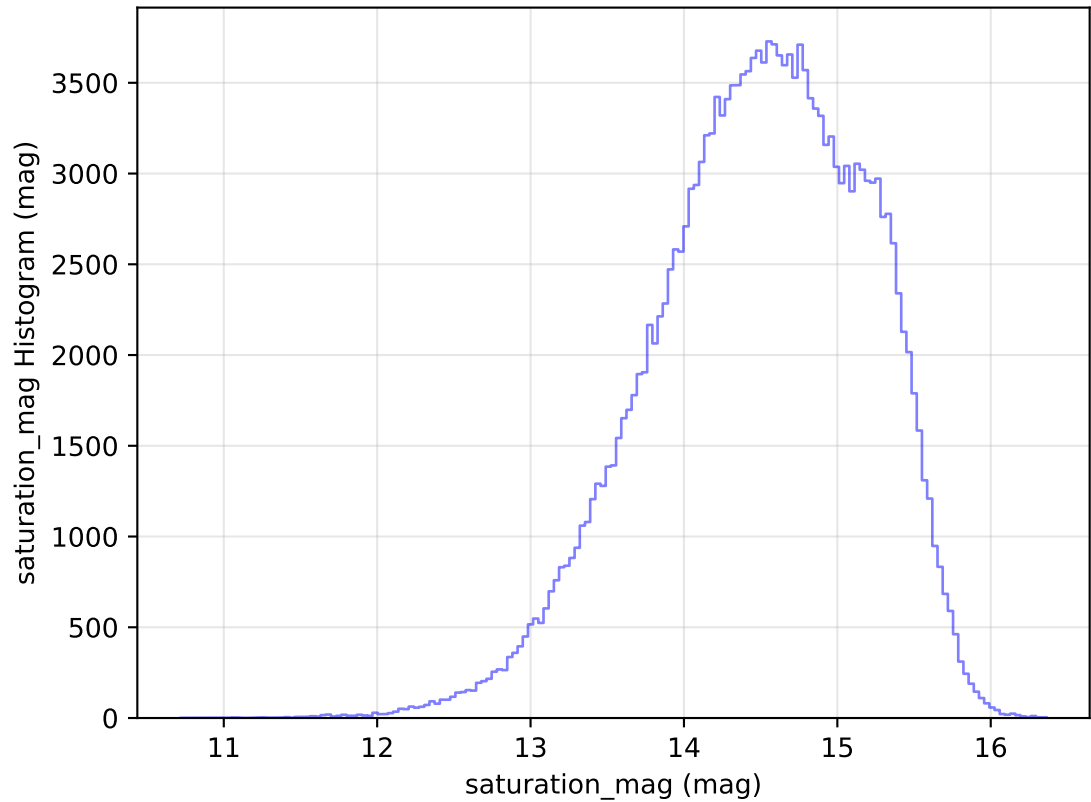
too_elab_r32_d2_ugrizy_v3.4_10yrs All sky g band: saturation_mag Histogram
