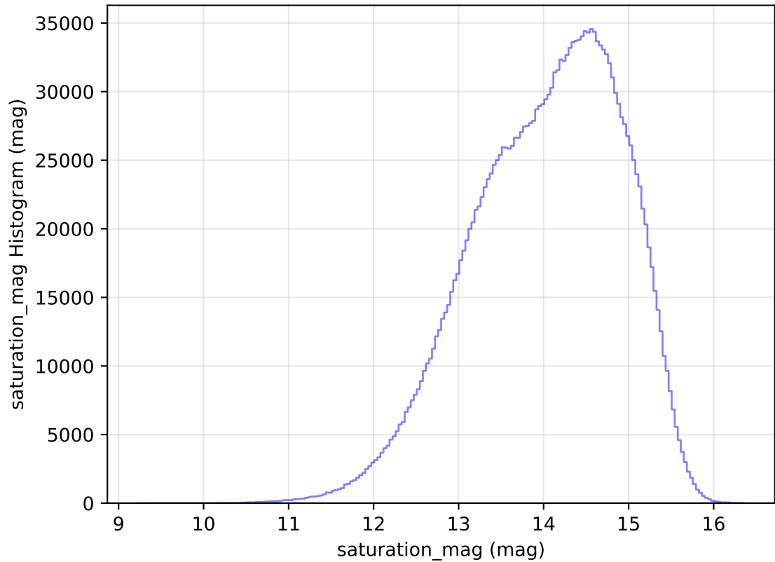
too_elab_r32_d2_ugrizy_v3.4_10yrs All sky all bands: saturation_mag Histogram
