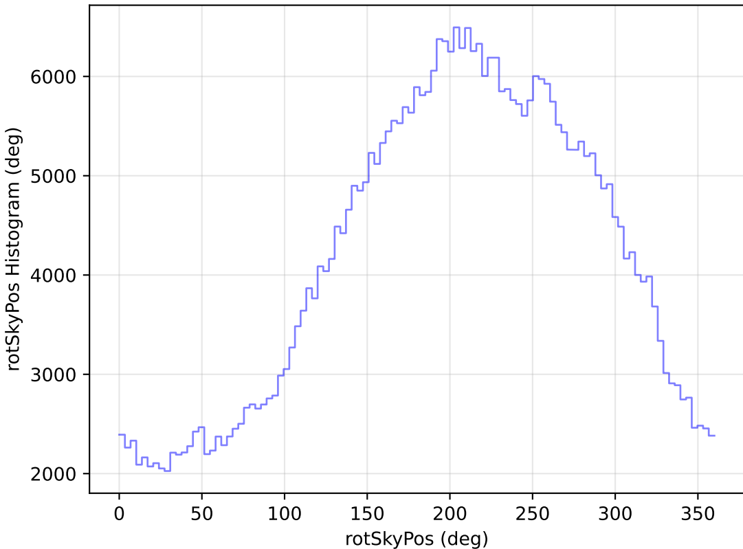
too_elab_r32_d2_ugrizy_v3.4_10yrs WFD z band: rotSkyPos Histogram
