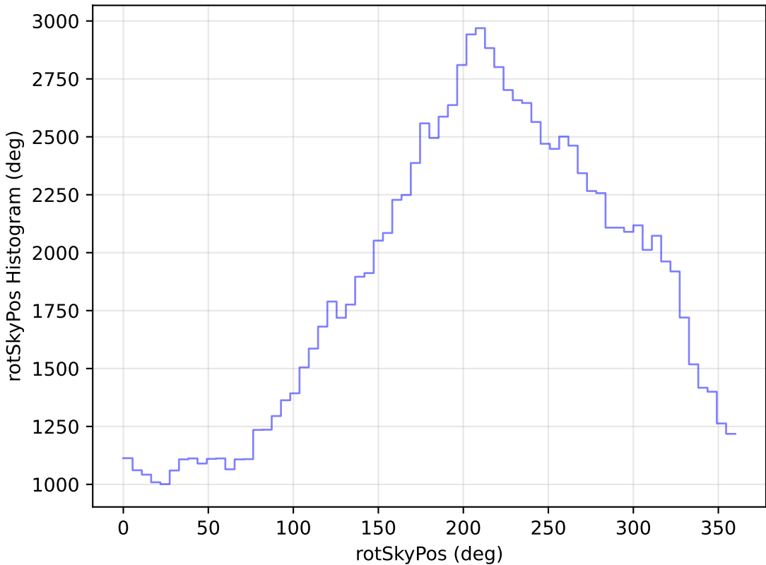
too_elab_r32_d2_ugrizy_v3.4_10yrs WFD u band: rotSkyPos Histogram
