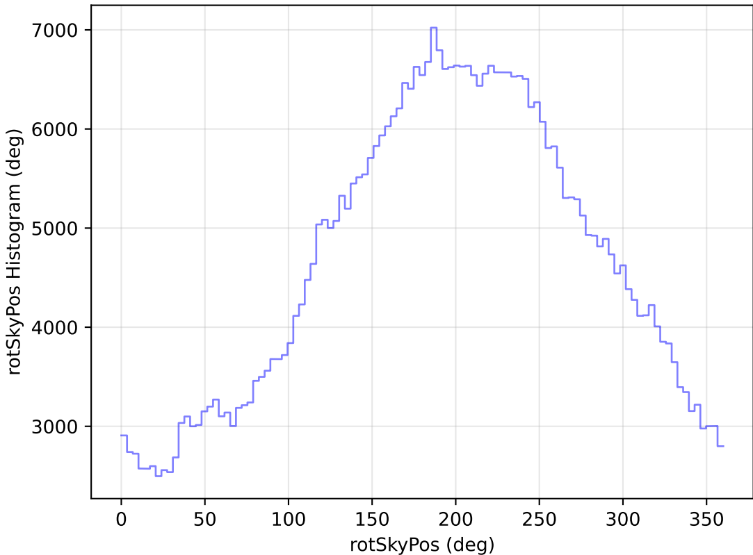
too_elab_r32_d2_ugrizy_v3.4_10yrs WFD r band: rotSkyPos Histogram
