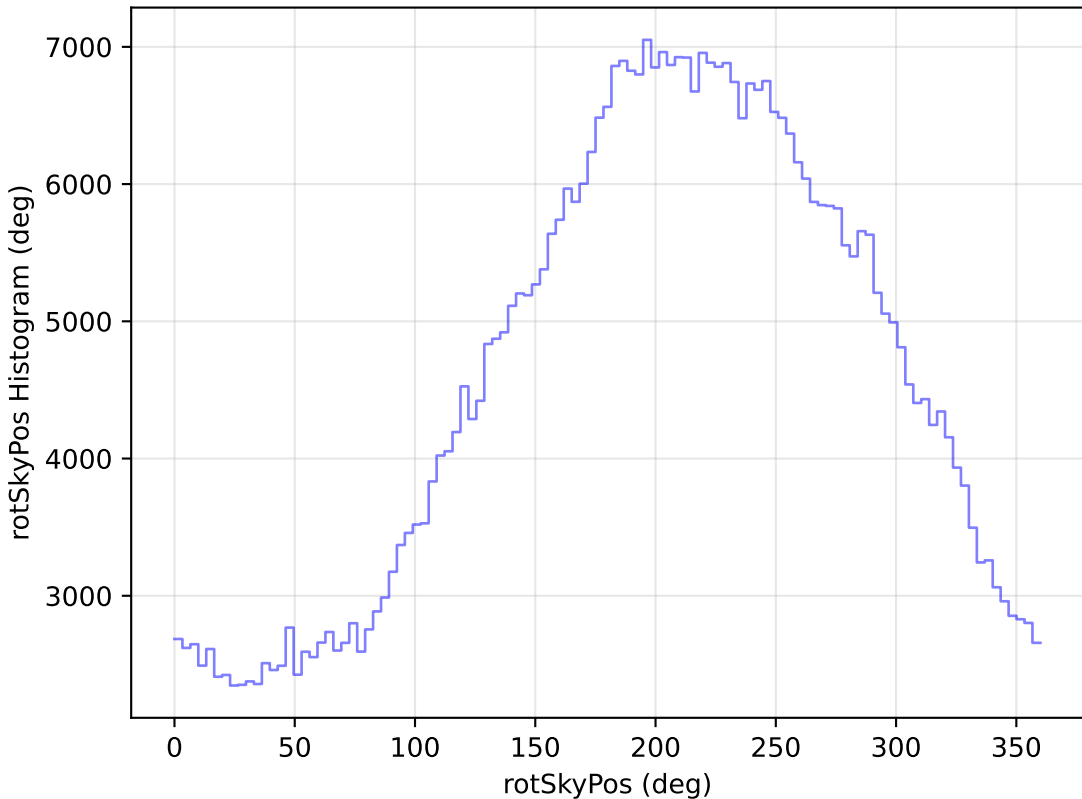
too_elab_r32_d2_ugrizy_v3.4_10yrs WFD i band: rotSkyPos Histogram
