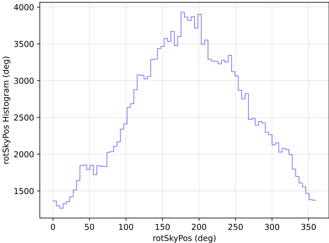
too_elab_r32_d2_ugrizy_v3.4_10yrs WFD g band: rotSkyPos Histogram
