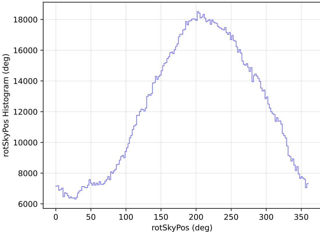
too_elab_r32_d2_ugrizy_v3.4_10yrs WFD all bands: rotSkyPos Histogram
