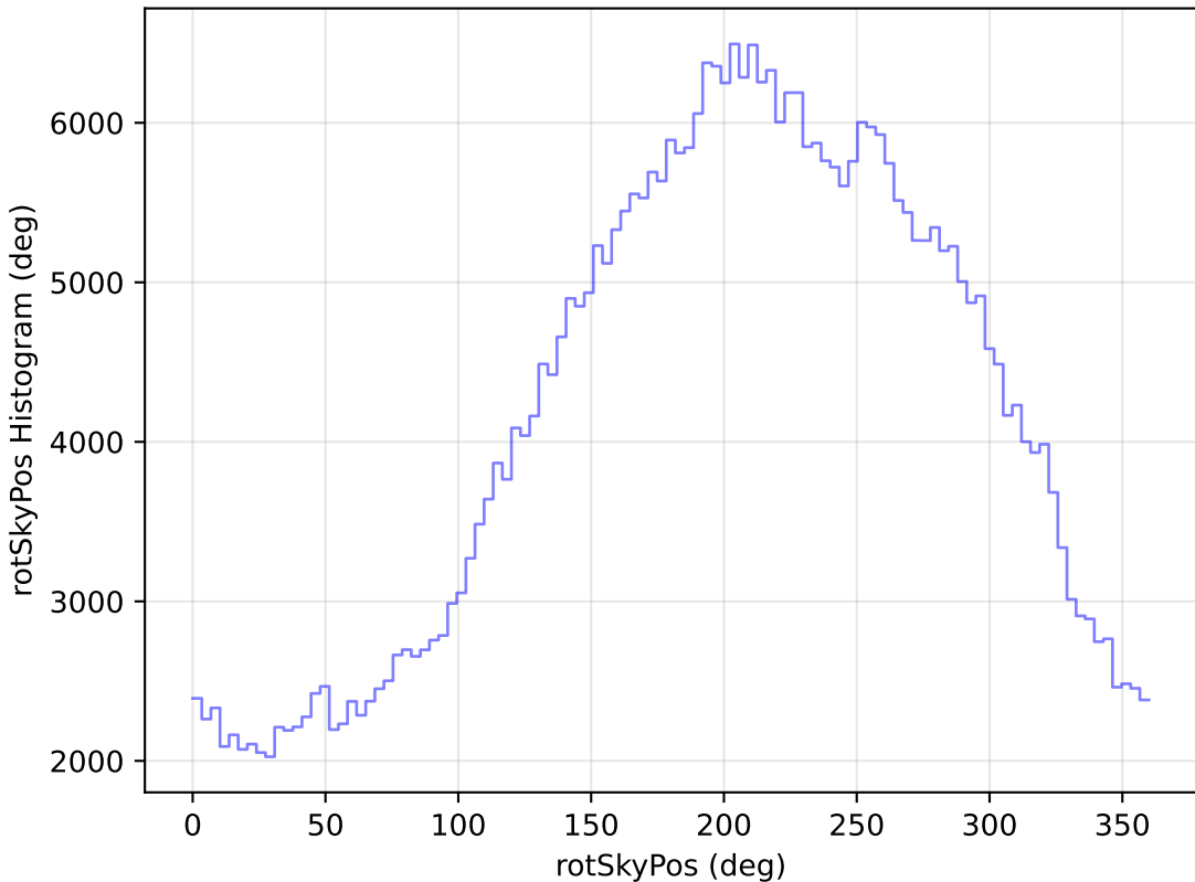
too_elab_r32_d2_ugrizy_v3.4_10yrs All sky z band: rotSkyPos Histogram
