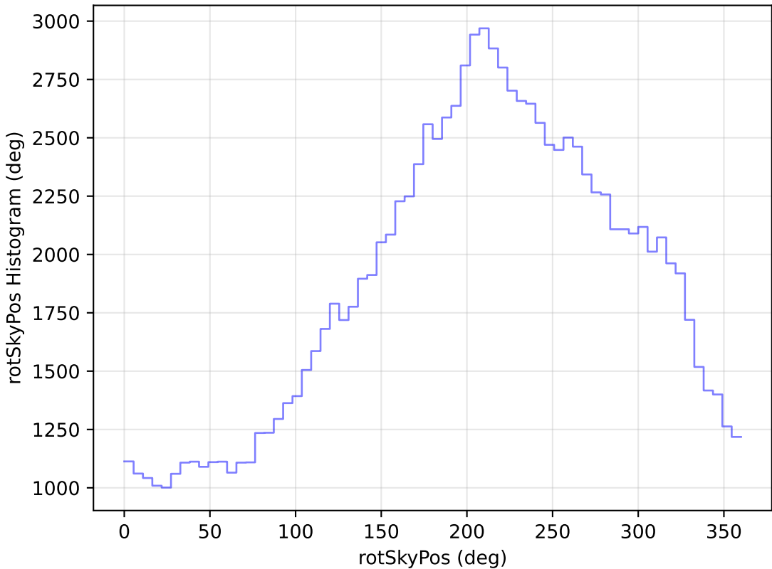
too_elab_r32_d2_ugrizy_v3.4_10yrs All sky u band: rotSkyPos Histogram
