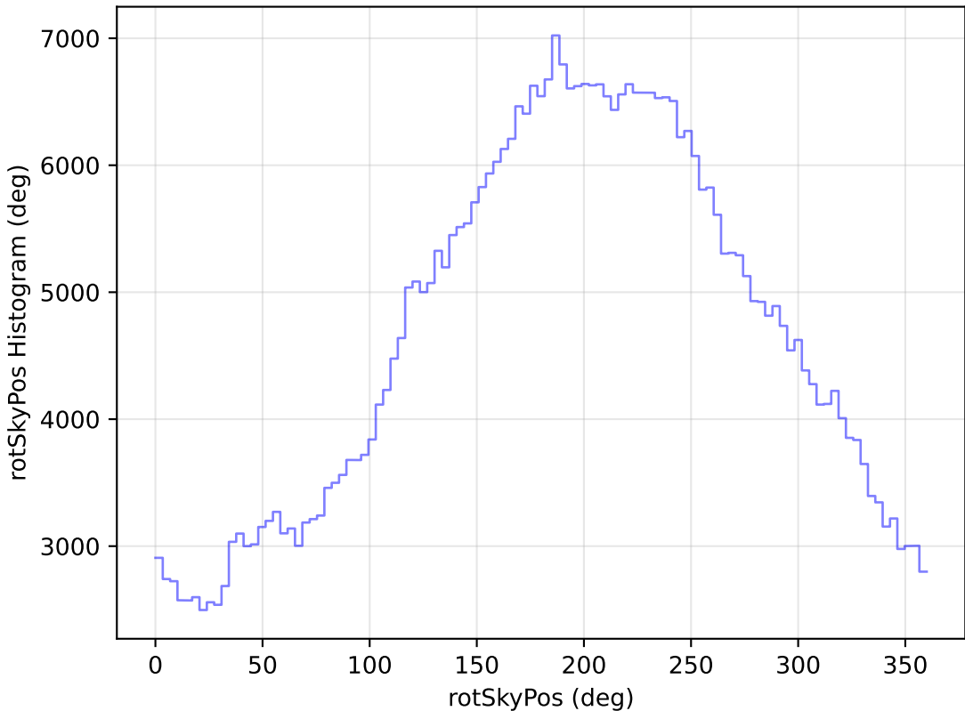
too_elab_r32_d2_ugrizy_v3.4_10yrs All sky r band: rotSkyPos Histogram
