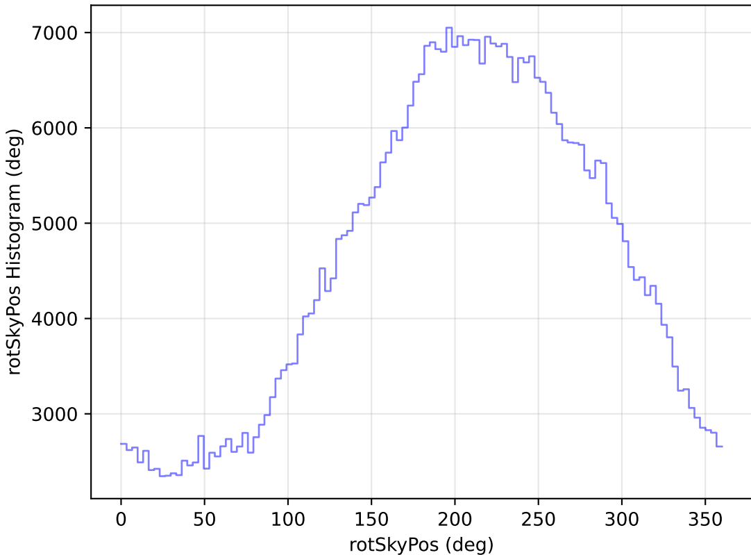
too_elab_r32_d2_ugrizy_v3.4_10yrs All sky i band: rotSkyPos Histogram
