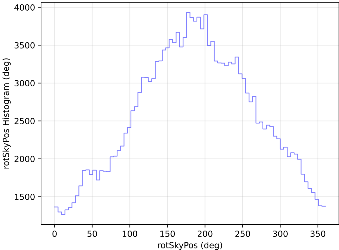
too_elab_r32_d2_ugrizy_v3.4_10yrs All sky g band: rotSkyPos Histogram
