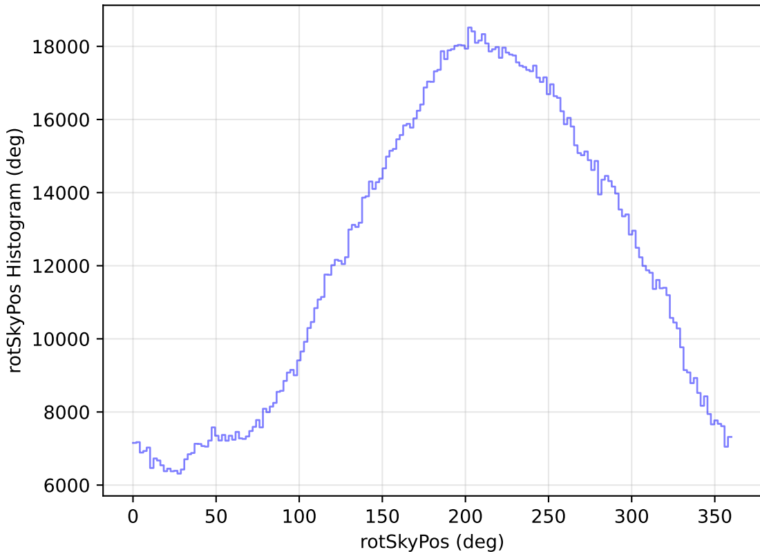
too_elab_r32_d2_ugrizy_v3.4_10yrs All sky all bands: rotSkyPos Histogram
