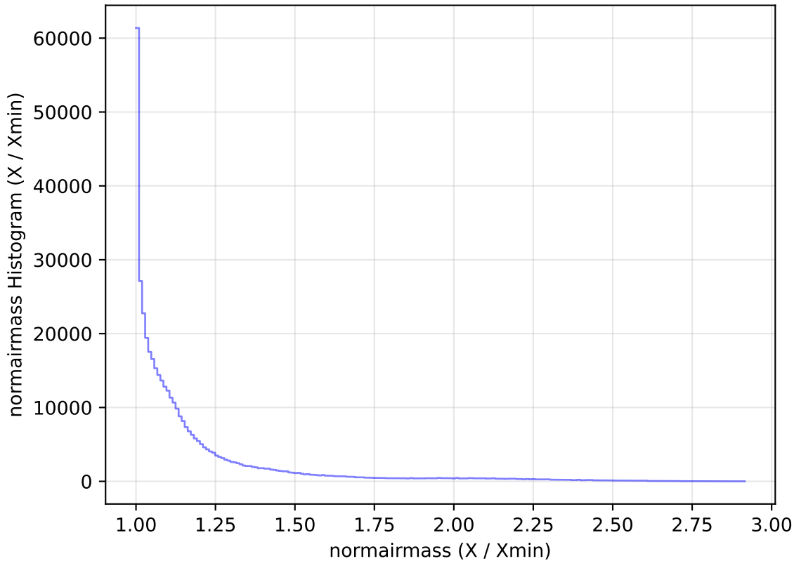
too_elab_r32_d2_ugrizy_v3.4_10yrs WFD z band: normairmass Histogram
