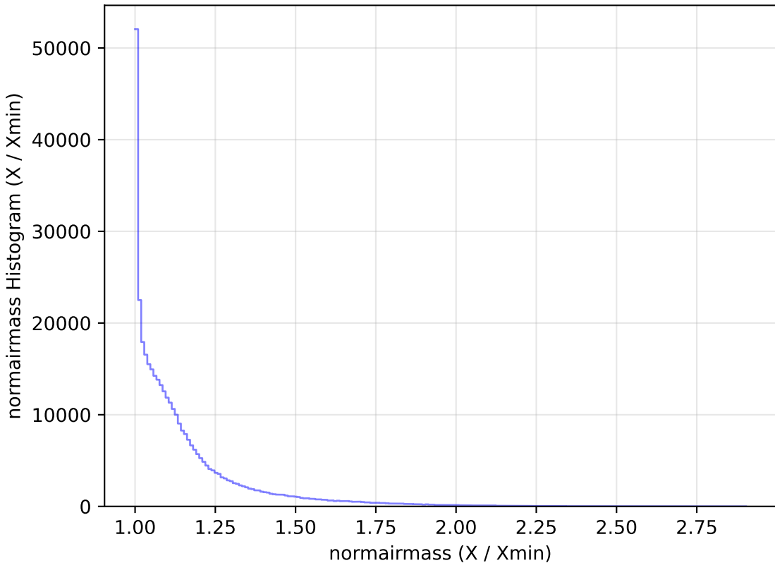
too_elab_r32_d2_ugrizy_v3.4_10yrs WFD y band: normairmass Histogram
