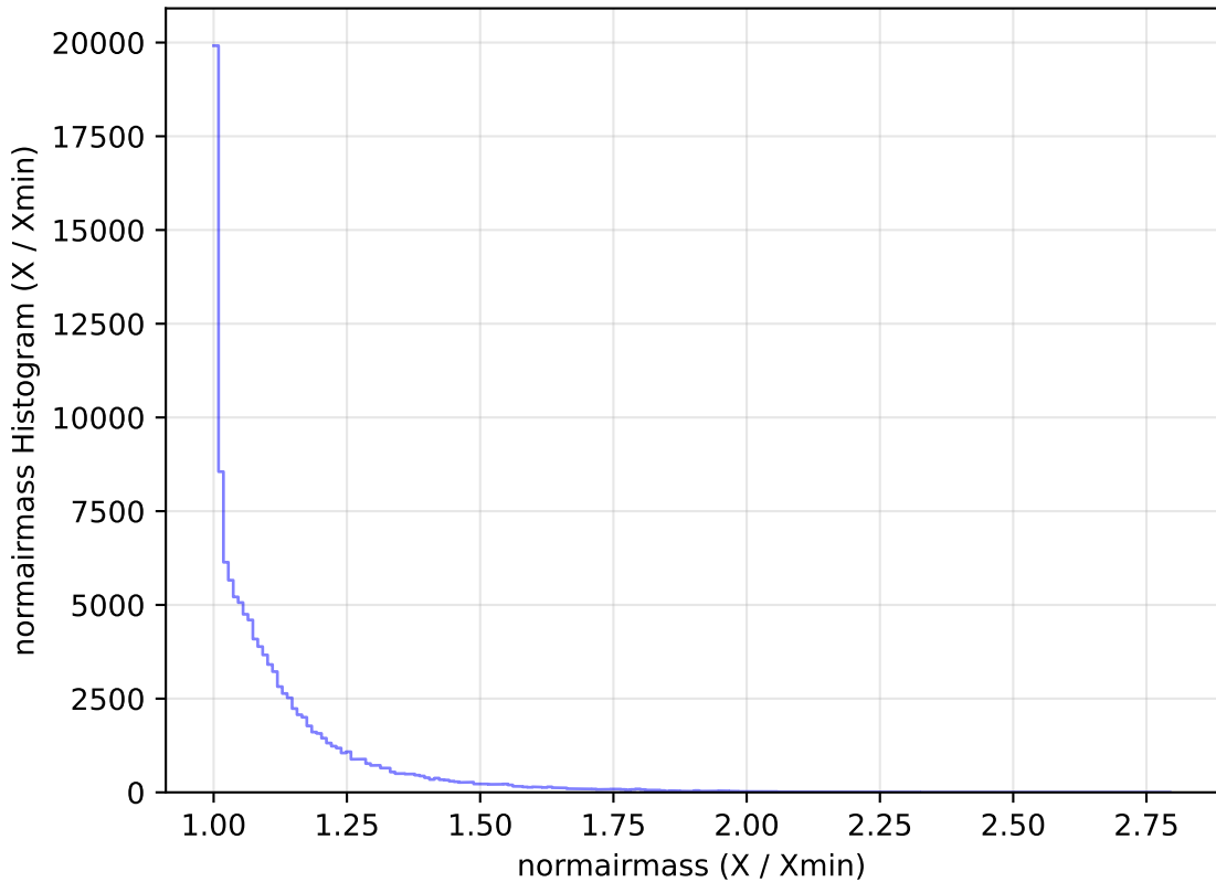
too_elab_r32_d2_ugrizy_v3.4_10yrs WFD u band: normairmass Histogram
