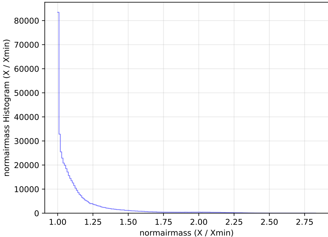
too_elab_r32_d2_ugrizy_v3.4_10yrs WFD r band: normairmass Histogram
