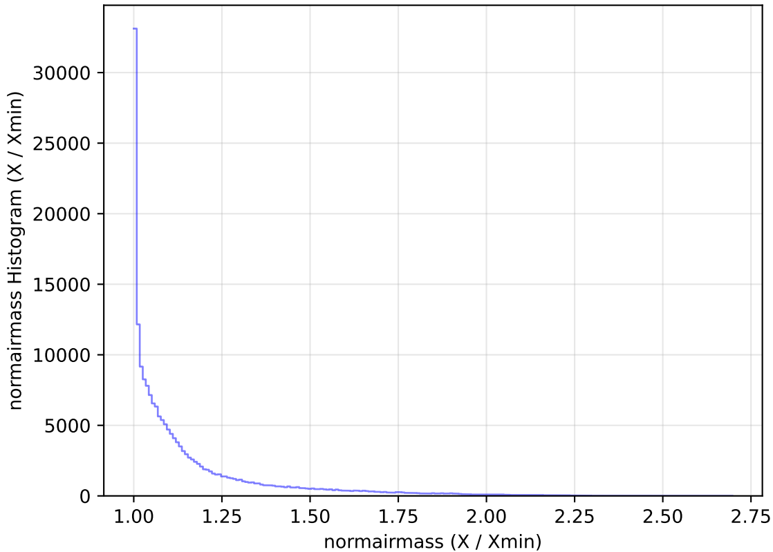
too_elab_r32_d2_ugrizy_v3.4_10yrs WFD g band: normairmass Histogram
