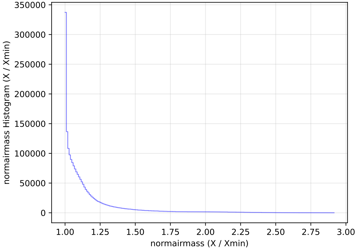
too_elab_r32_d2_ugrizy_v3.4_10yrs WFD all bands: normairmass Histogram
