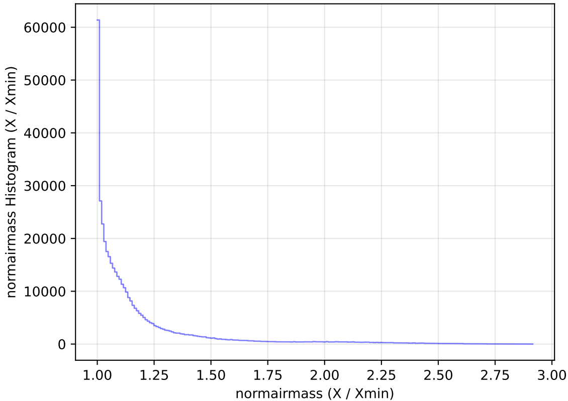
too_elab_r32_d2_ugrizy_v3.4_10yrs All sky z band: normairmass Histogram
