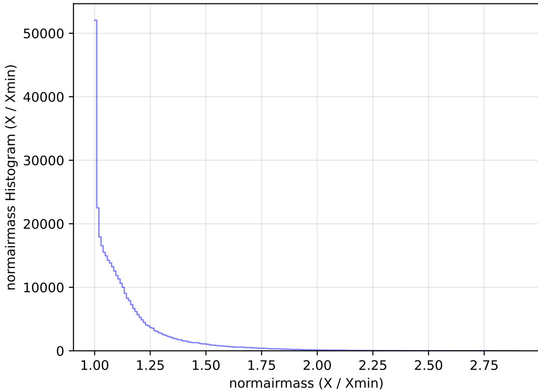
too_elab_r32_d2_ugrizy_v3.4_10yrs All sky y band: normairmass Histogram
