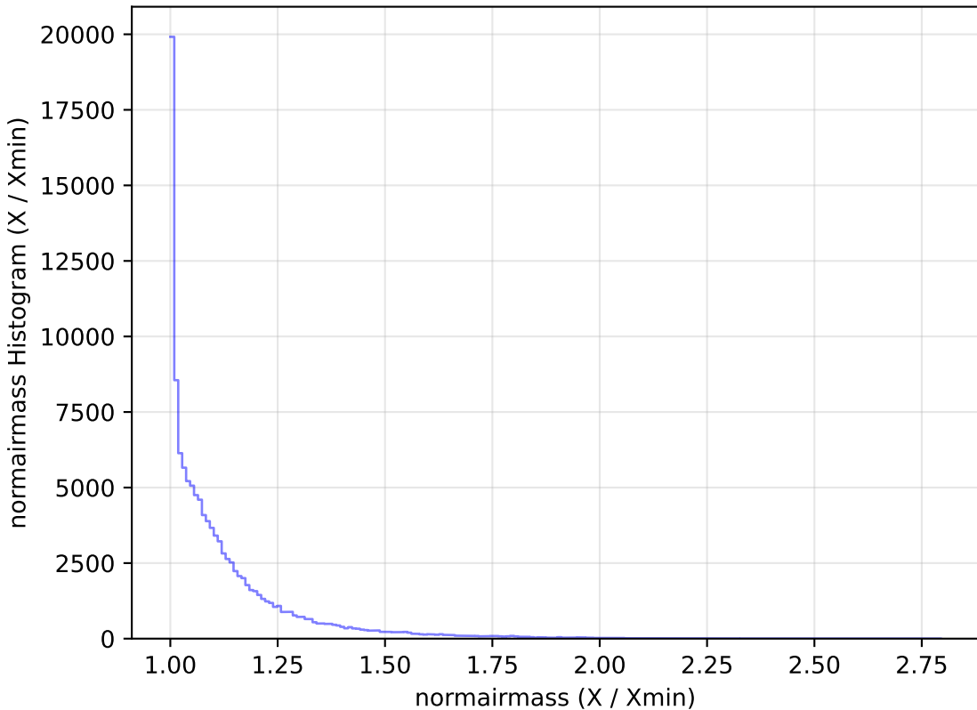
too_elab_r32_d2_ugrizy_v3.4_10yrs All sky u band: normairmass Histogram
