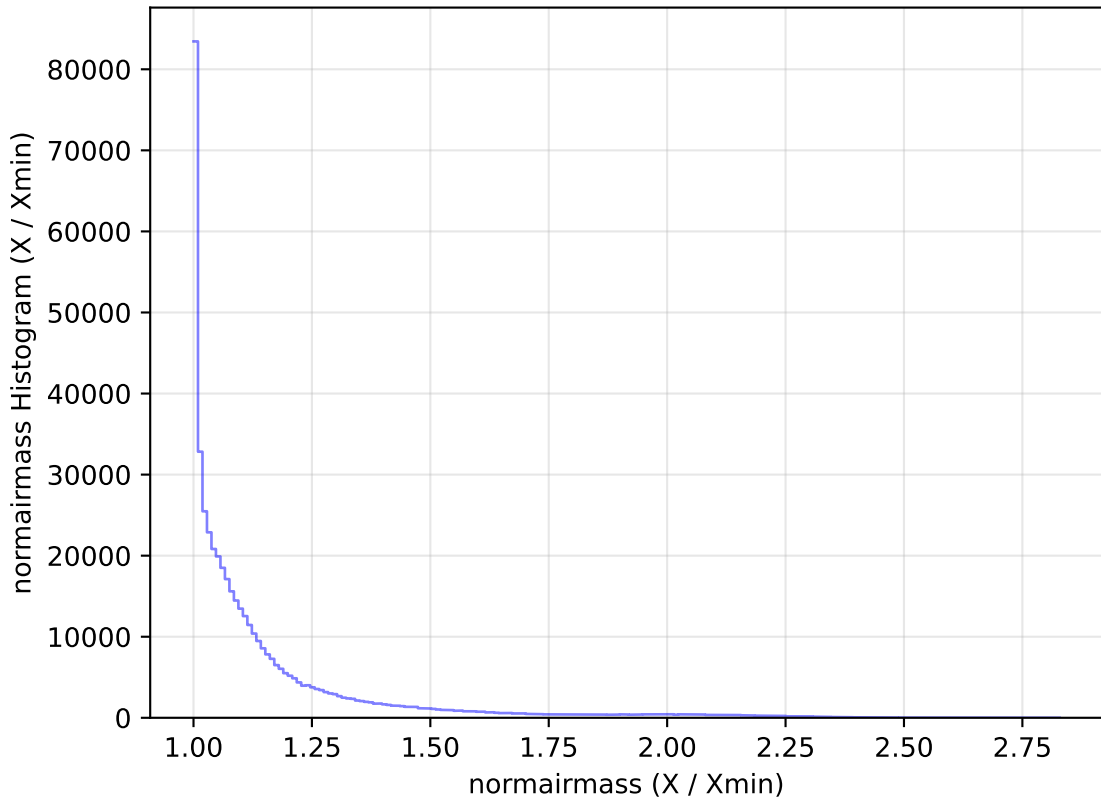
too_elab_r32_d2_ugrizy_v3.4_10yrs All sky r band: normairmass Histogram
