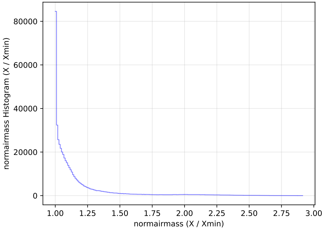
too_elab_r32_d2_ugrizy_v3.4_10yrs All sky i band: normairmass Histogram
