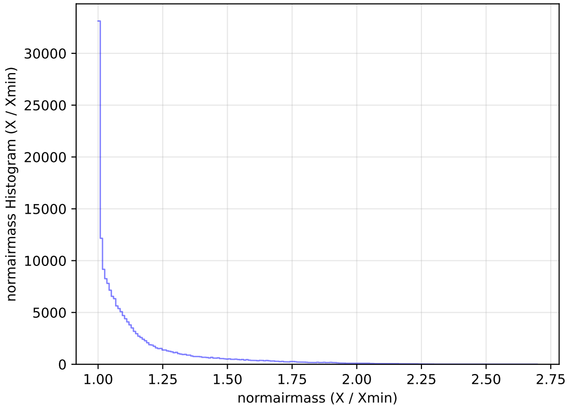
too_elab_r32_d2_ugrizy_v3.4_10yrs All sky g band: normairmass Histogram
