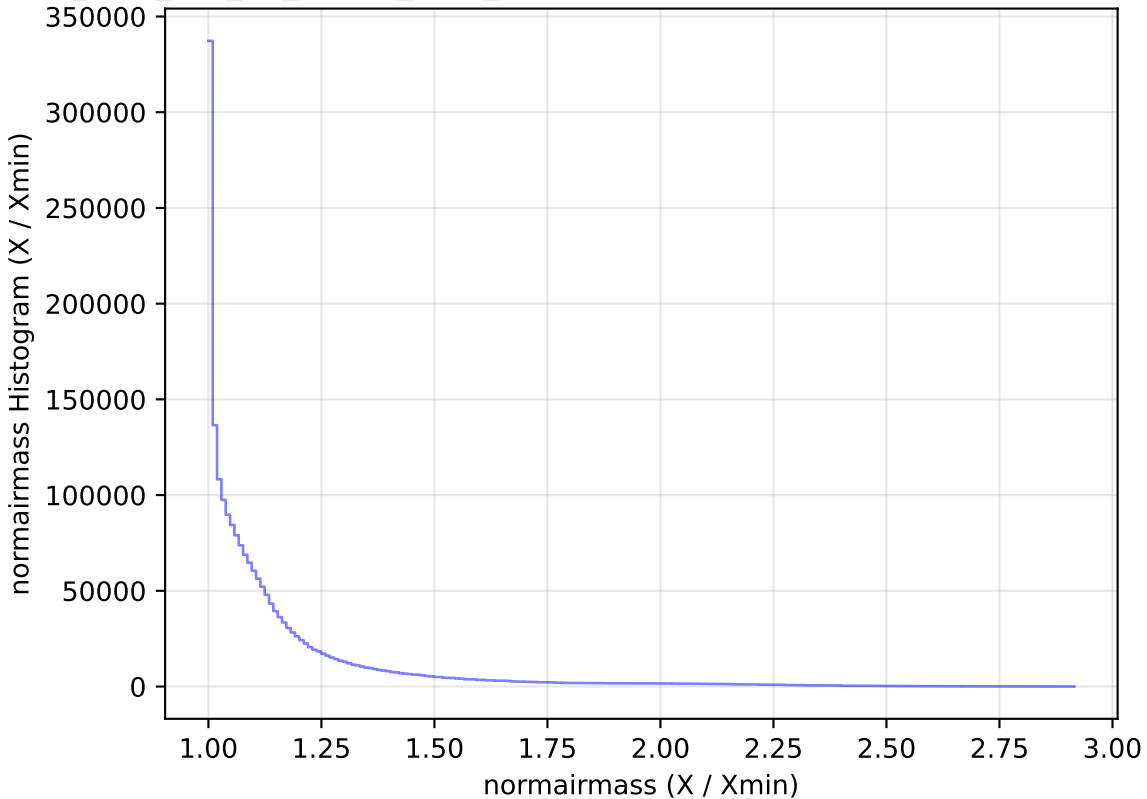
too_elab_r32_d2_ugrizy_v3.4_10yrs All sky all bands: normairmass Histogram
