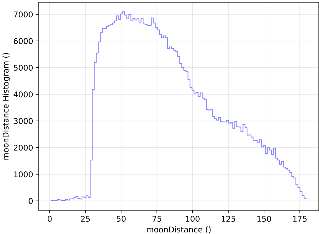
too_elab_r32_d2_ugrizy_v3.4_10yrs WFD z band: moonDistance Histogram
