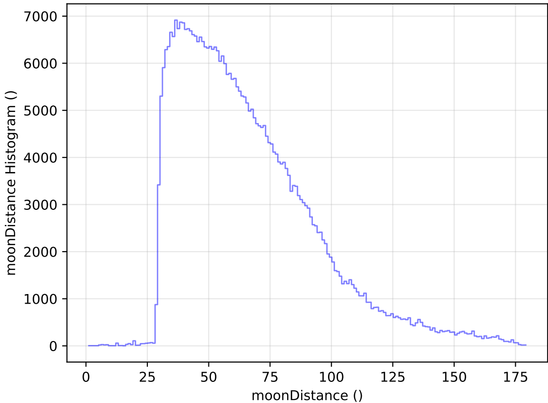
too_elab_r32_d2_ugrizy_v3.4_10yrs WFD y band: moonDistance Histogram
