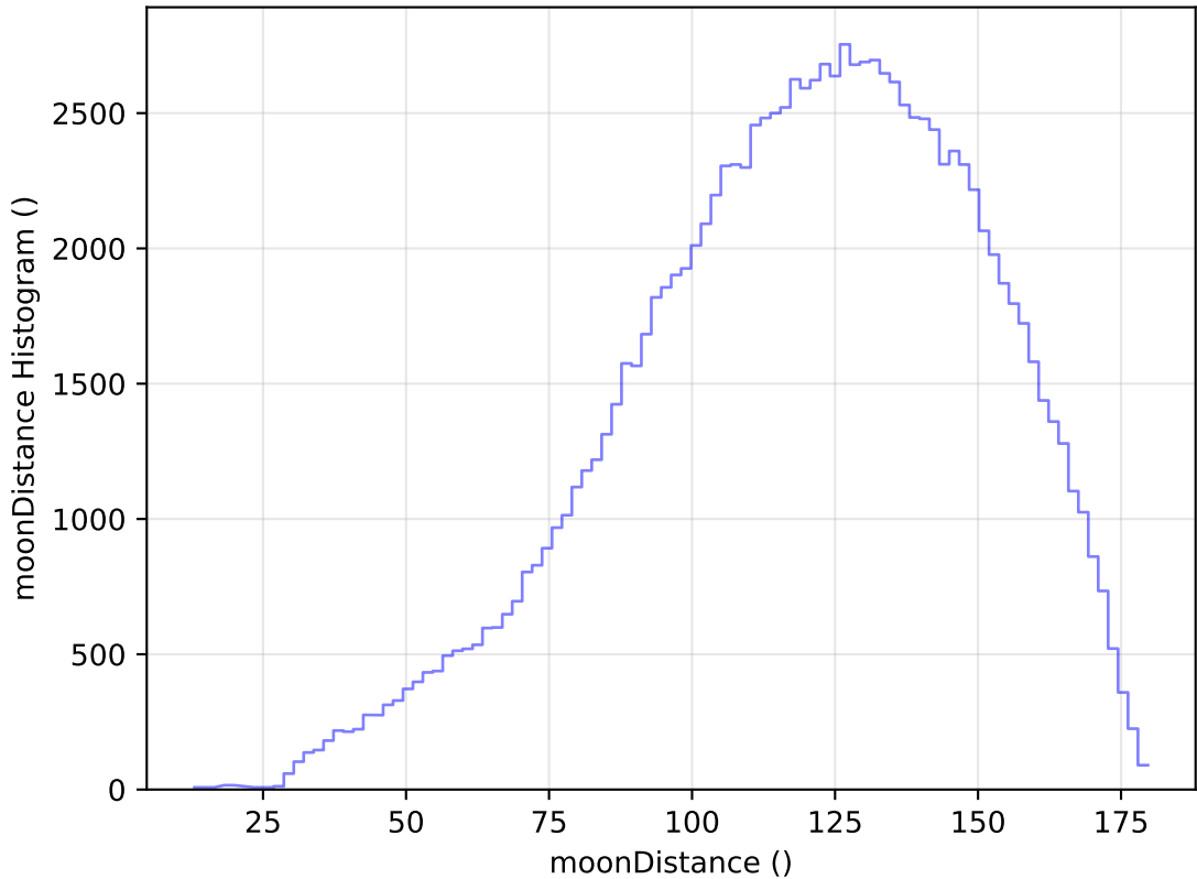
too_elab_r32_d2_ugrizy_v3.4_10yrs WFD u band: moonDistance Histogram
