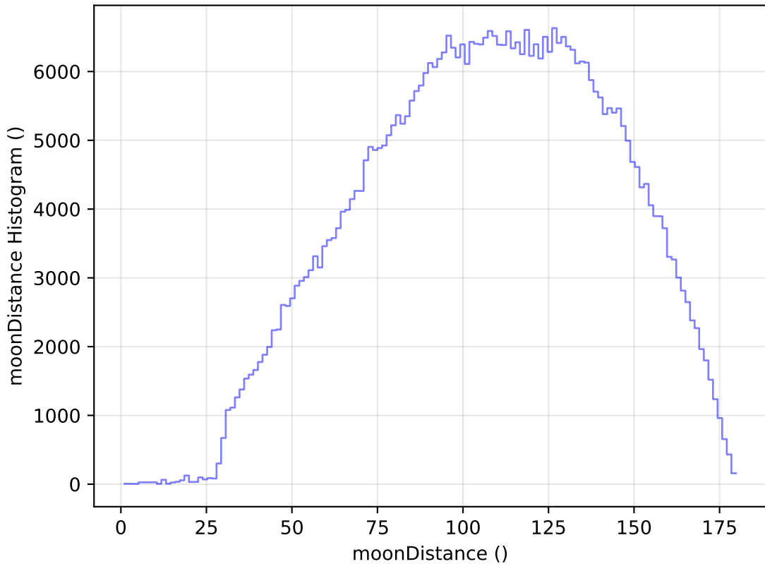
too_elab_r32_d2_ugrizy_v3.4_10yrs WFD r band: moonDistance Histogram
