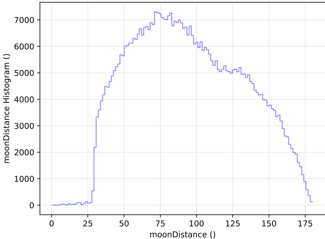
too_elab_r32_d2_ugrizy_v3.4_10yrs WFD i band: moonDistance Histogram
