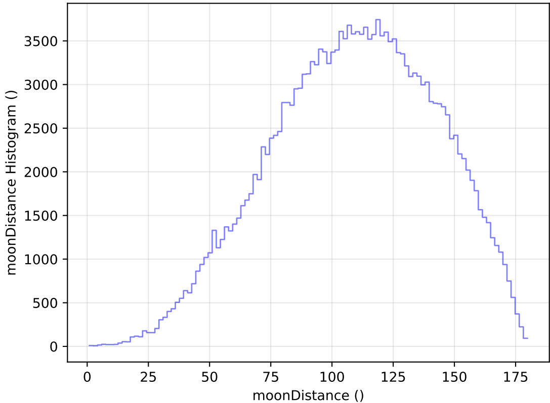
too_elab_r32_d2_ugrizy_v3.4_10yrs WFD g band: moonDistance Histogram
