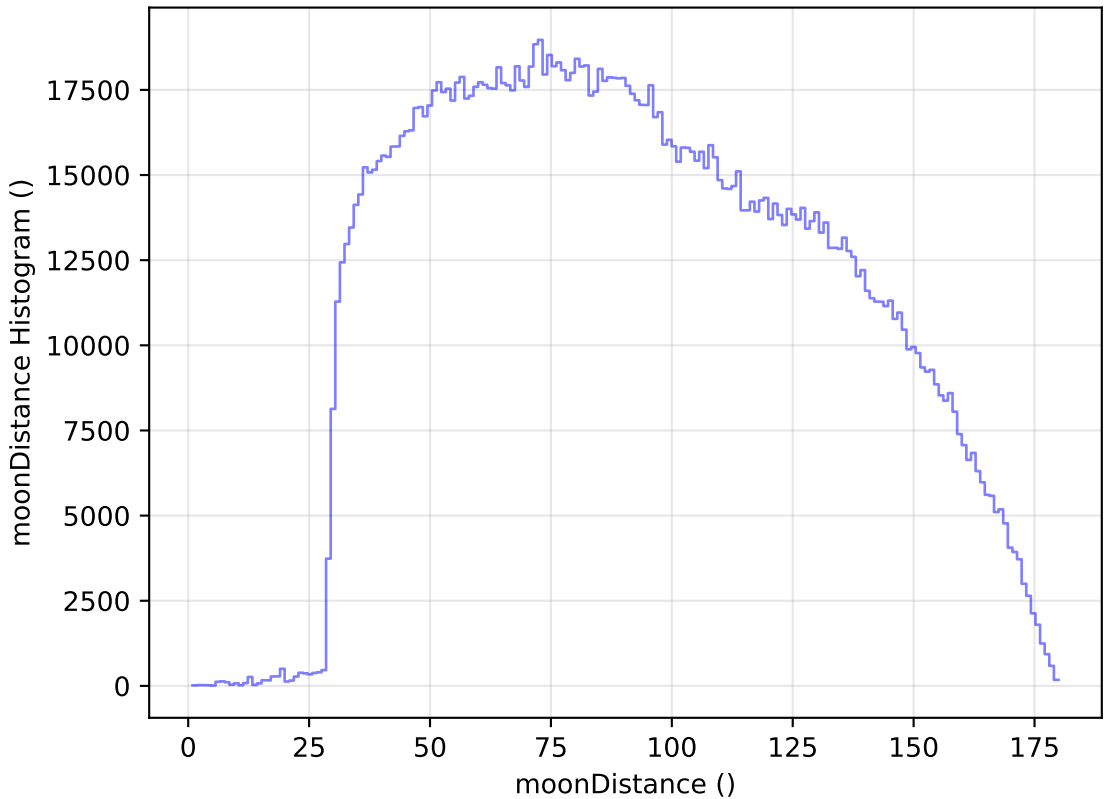
too_elab_r32_d2_ugrizy_v3.4_10yrs WFD all bands: moonDistance Histogram
