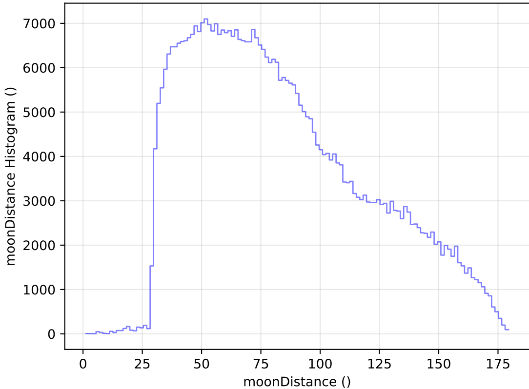
too_elab_r32_d2_ugrizy_v3.4_10yrs All sky z band: moonDistance Histogram
